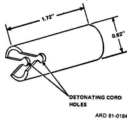
Figure 4-17. Detonating cord connector,
